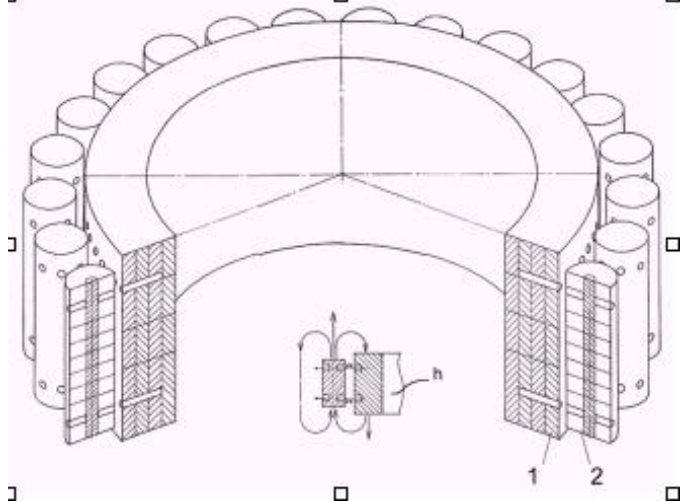
Fig.1. Variant of one-ring converter.
