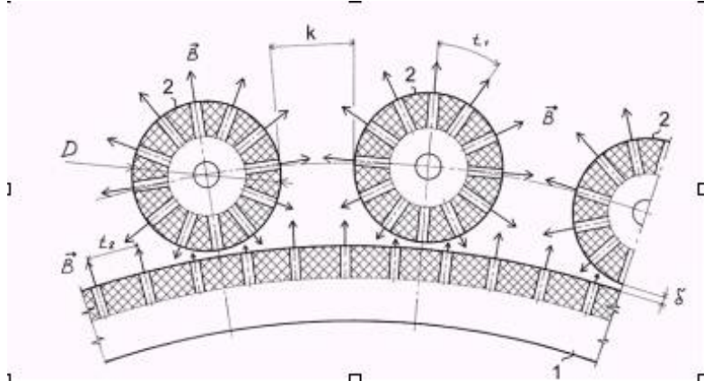
Fig.2. A way of organization of magnetic gearing stator and rollers.
